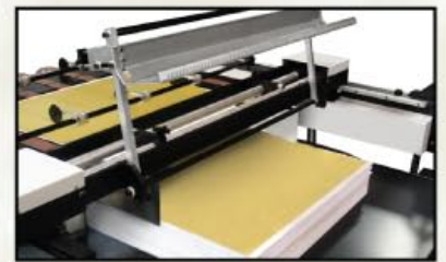
Adjustable Back-stop (up)
